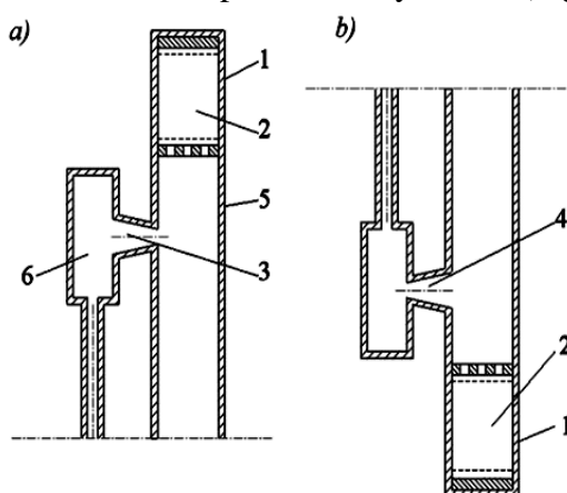
Figure 1 a, b – Combined friction belt of a disc-shoe brake with a forced air-nano-liquid cooling system: 1 – friction belt; 2 – zones of overlapping by friction linings; 3 – confusers; 4 – diffusers; 5, 6 – zones: evaporation, condensation; a and b – upper and lower parts of the tubular system, which is not filled with nano-liquid
