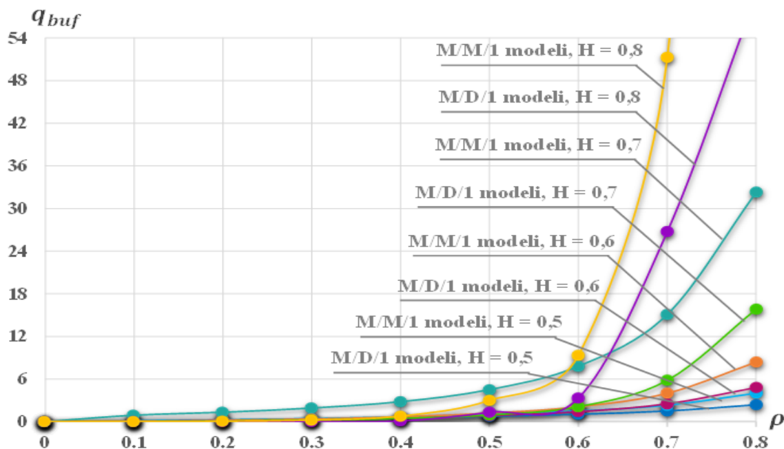
Figure 1 – The dependency of the memory buffer size in NGN networks on the network load
